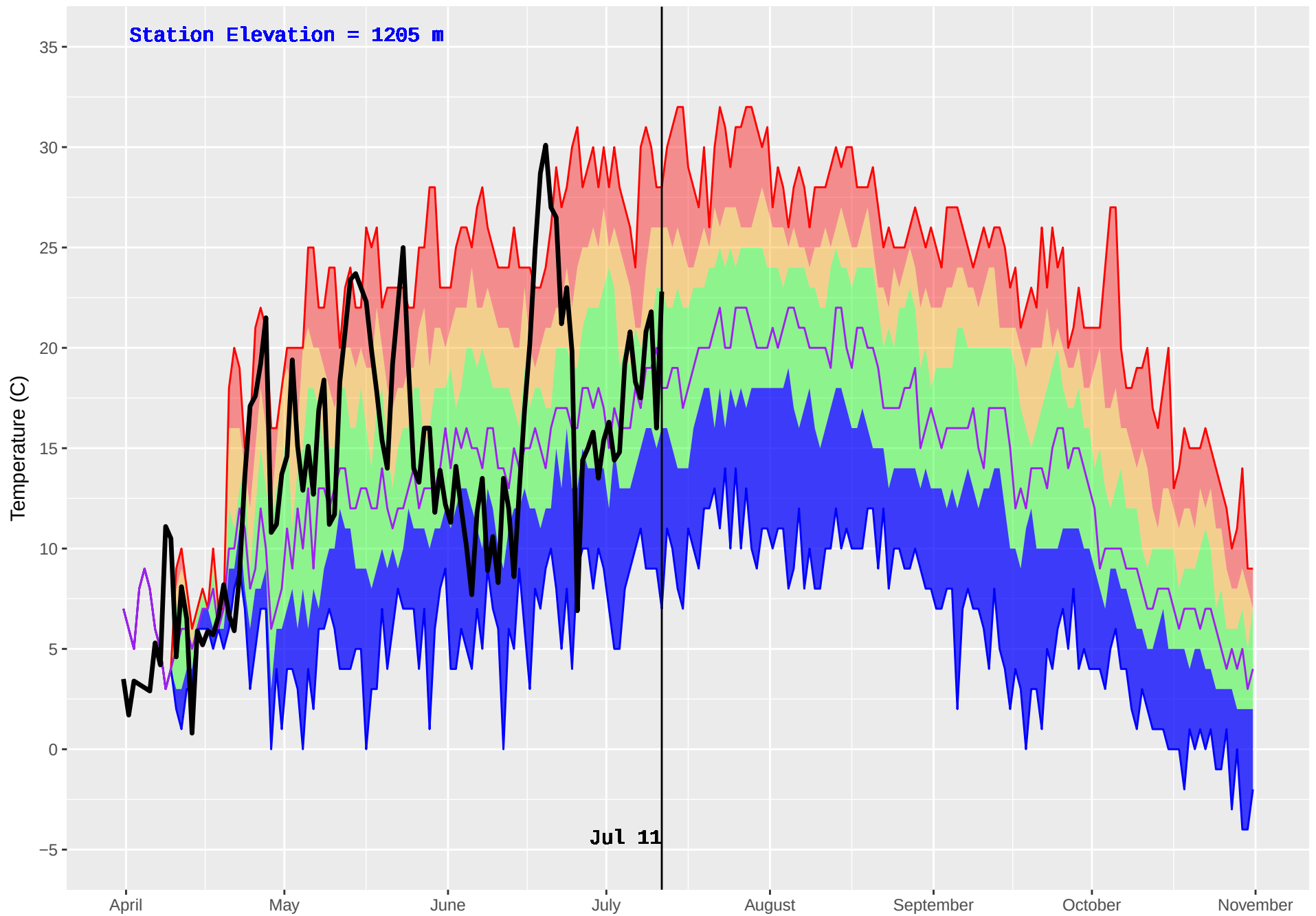
GWYNETH LAKE (309) : Historical (1986–2016) and Current (2018) Noon Temperature
