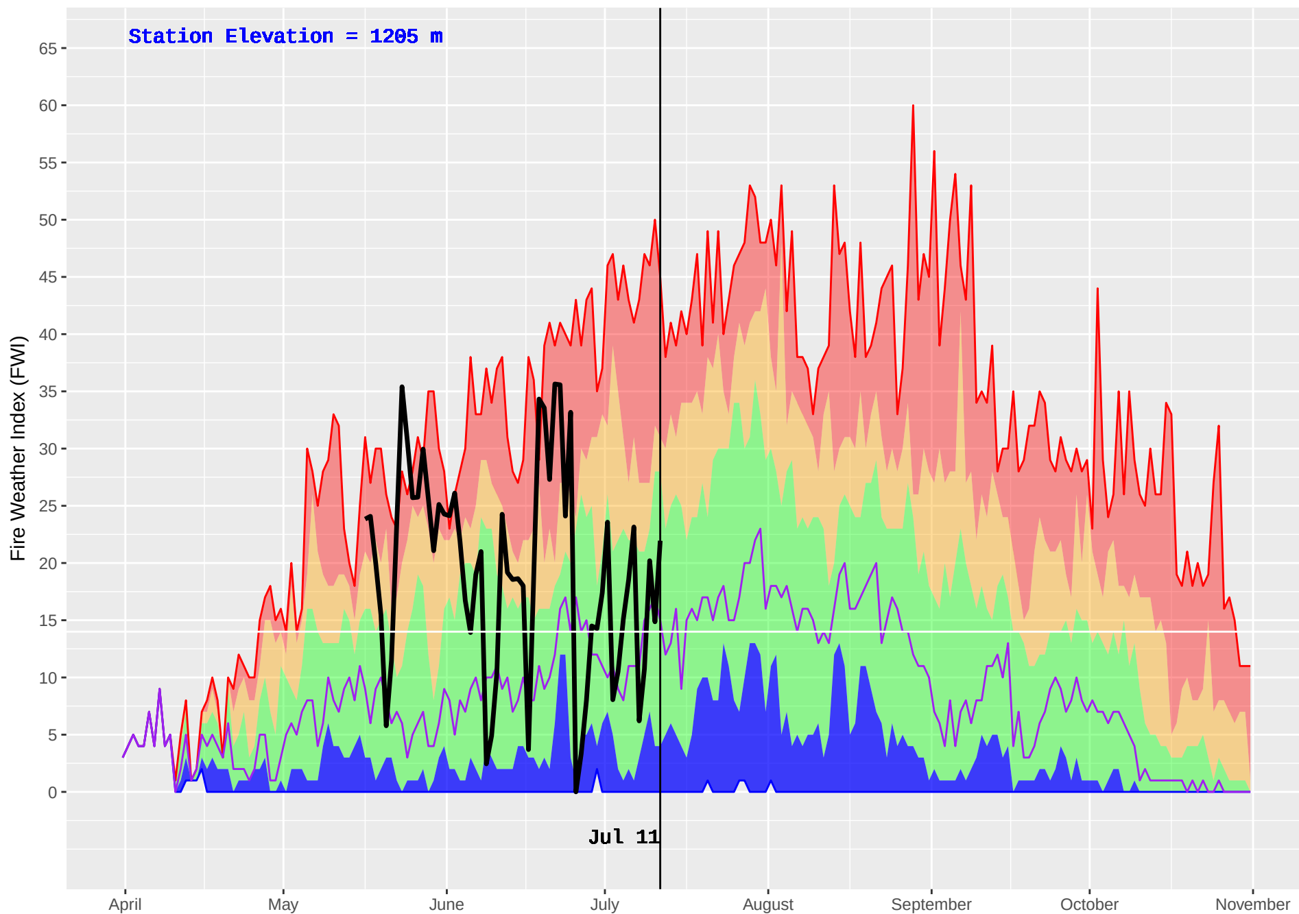
GWYNETH LAKE (309) : Historical (1986–2016) and Current (2018) Noon Fire Weather Index (FWI)
