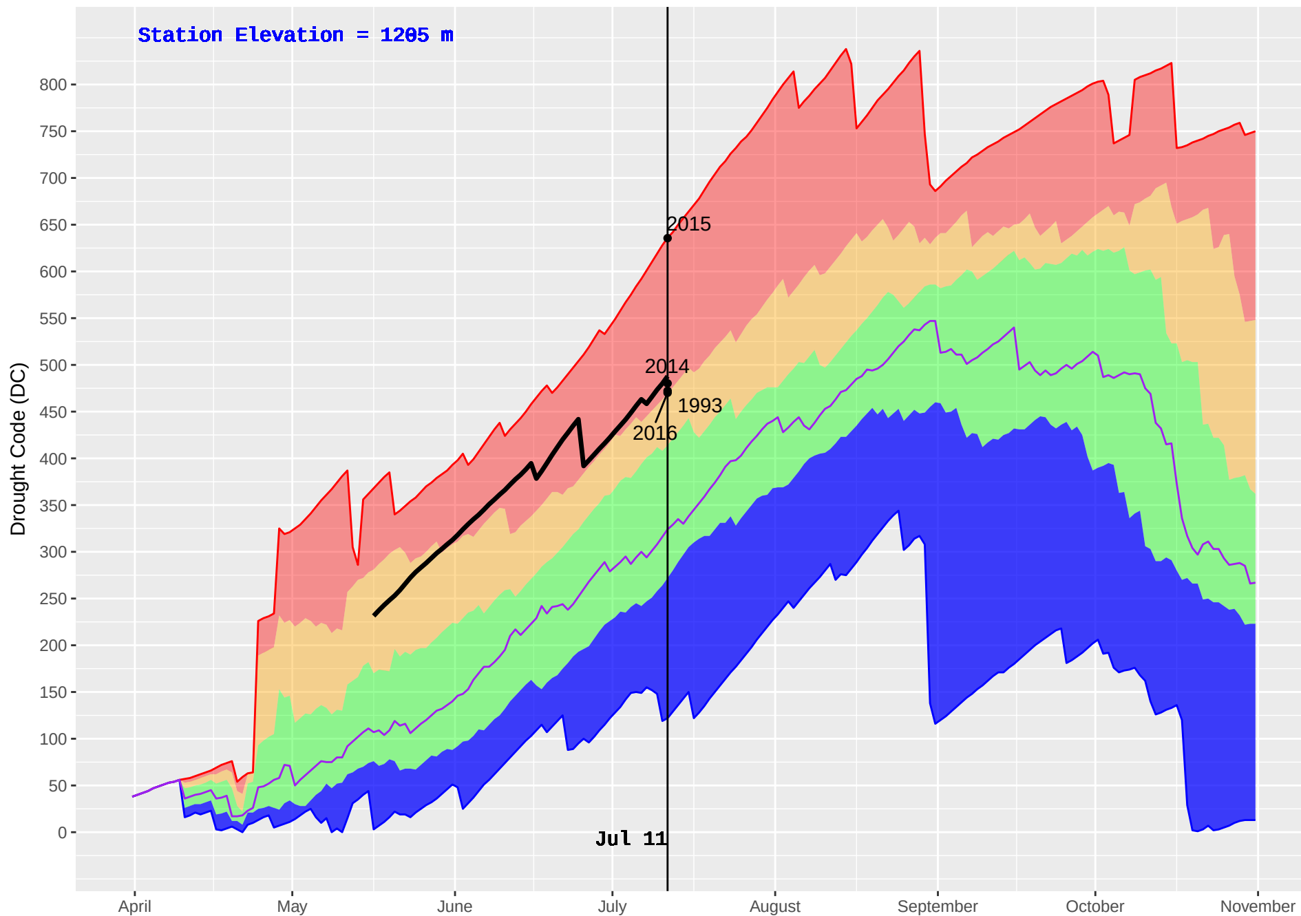
GWYNETH LAKE (309) : Historical (1986–2016) and Current (2018) Noon Drought Code (DC)
