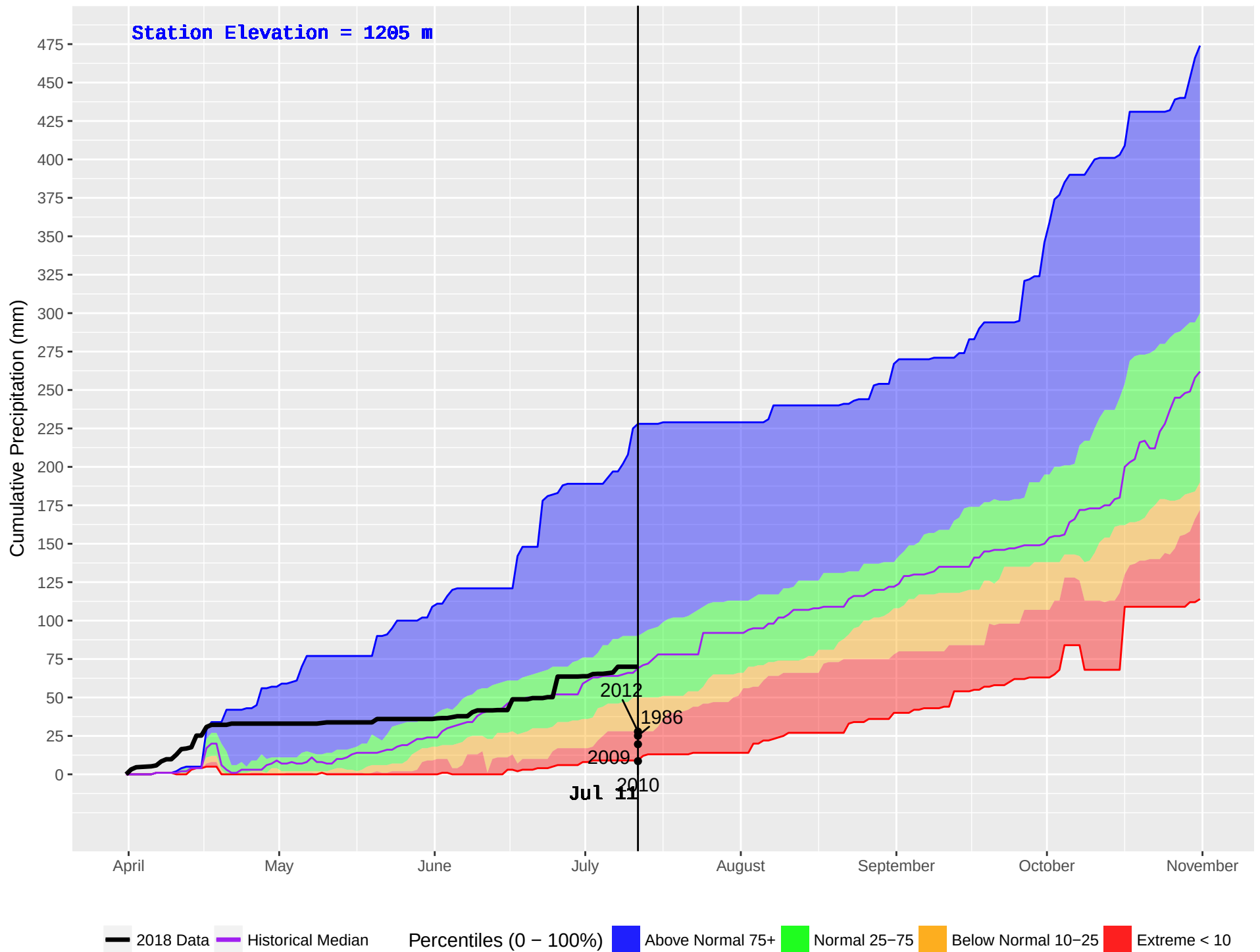
GWYNETH LAKE (309) : Historical (1986–2016) and Current (2018) Noon Cumulative Precipitation
